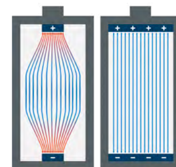
TAB DESIGN
